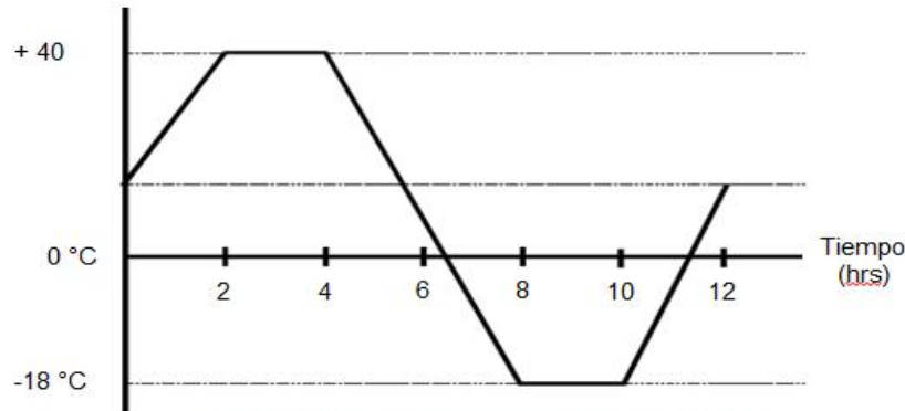
Fig. 6. IEC 61300-2-22, IEC 60068-2-14: Temperature Cycle Aging
